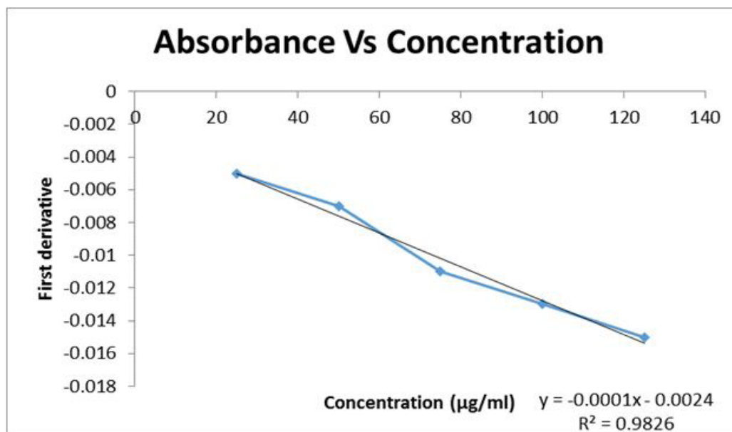
Figure 6: Calibration Curve of Metformin HCl at 272 nm in Methanol Solution Within the range of 25 to 125 µg/ml the drug obeyed Beer's law
